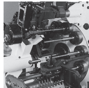
Trimming machine
